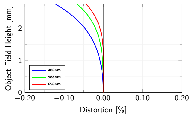
Object Field Height vs. Distortion, from the optical axis to the corner of the field of view
