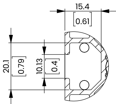
T-Slot DETAIL A SCALE 1:1
