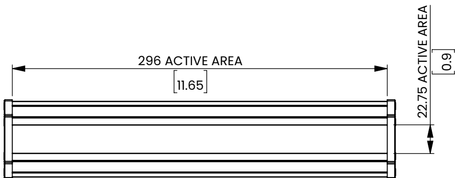
T-SLOT DETAIL A SCALE 1:1
