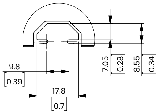
T-SLOT DETAIL A SCALE 1:1
