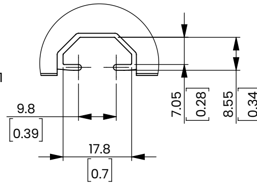
T-SLOT DETAIL A SCALE 1:1
