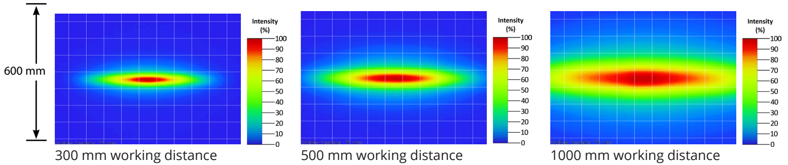
Line ( 10^{\circ} \times 50^{\circ} ) beam patterns Grid set to 75 mm
