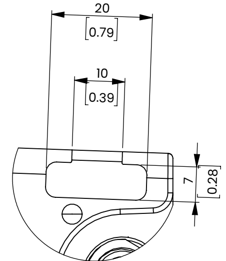
T-SLOT DETAIL A SCALE 4:3
