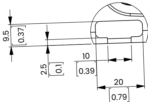
T-SLOT DETAIL A SCALE 1:1
