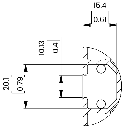
T-Slot DETAIL A SCALE 1:1
