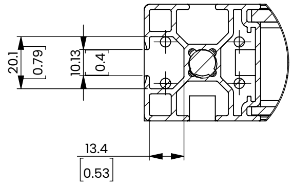
T-SLOT DETAIL A SCALE 2:3
