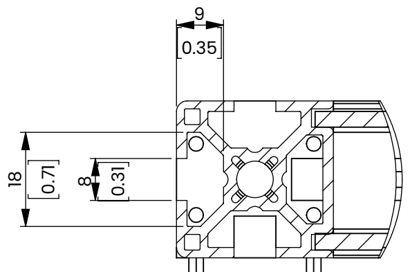
T-Slot DETAIL A SCALE 1:1
