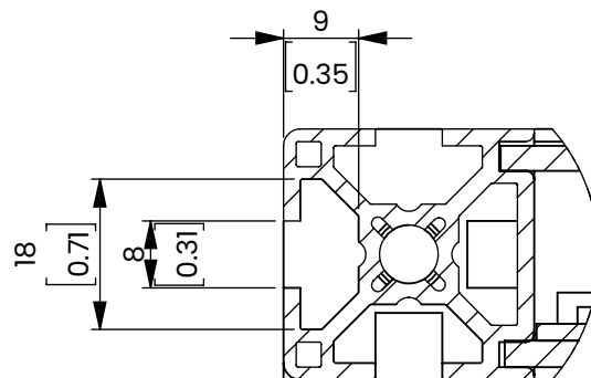
T-SLOT DETAIL A SCALE 1:1
