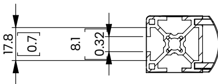
T-SLOT DETAIL A SCALE 1:2 (1 : 2)
